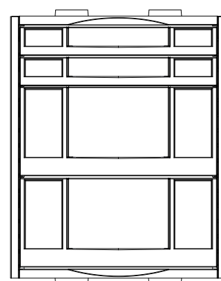
Kit tiroirs 150-50 2 drawer H150mm and 2 drawer H50mm kit
